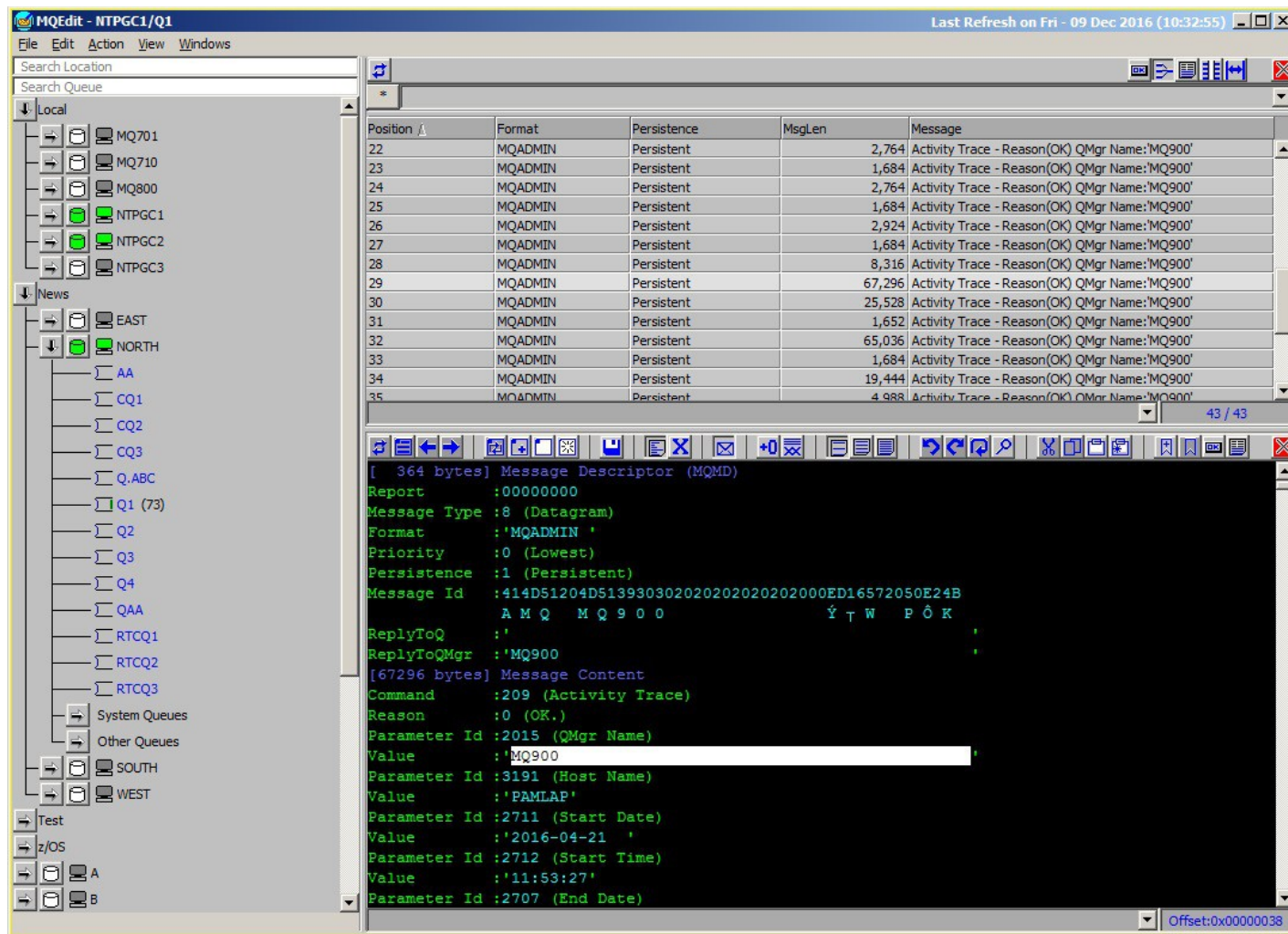
Figure 1: Main Window
